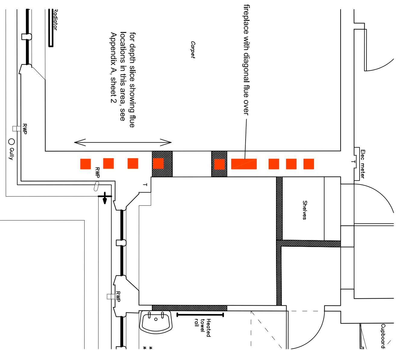
SAMPLE DATA, Location of Chimney Flues using GPR
